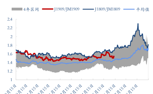
图8：J1909/JM1909
