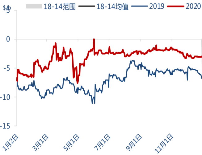
图3：WTI-Brent
