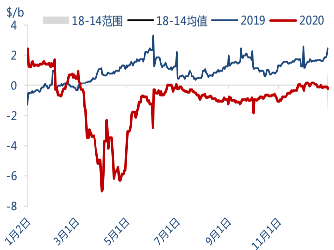
图6：Brent C1-C3
